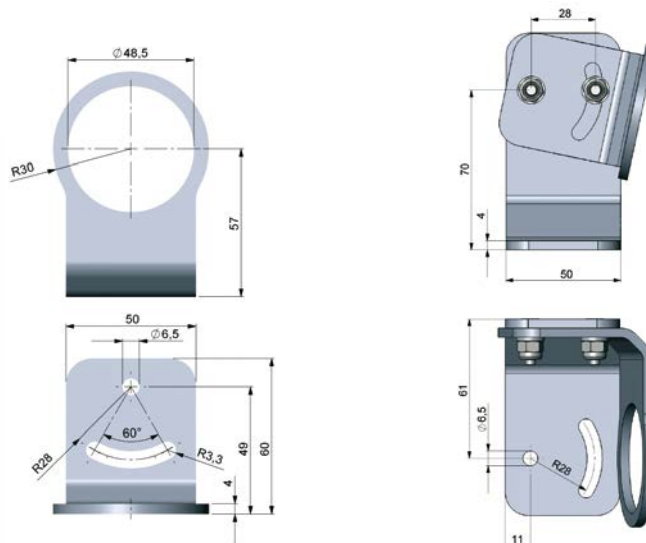
TM-FB-CTL Mounting bracket (fixed); included in CTL scope of supply
